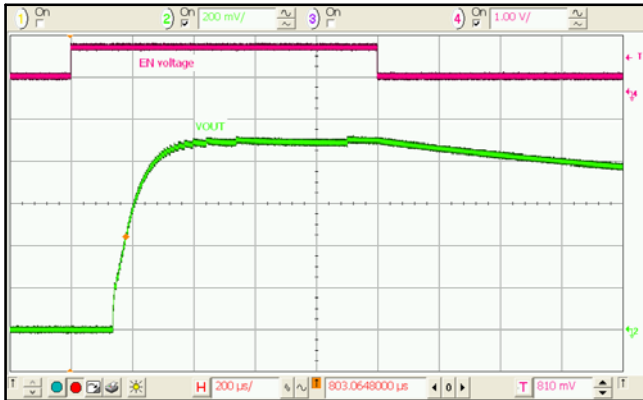
Figure 29. Startup / Shutdown, No Load, V_{OUT}=0.9\text{ V}
