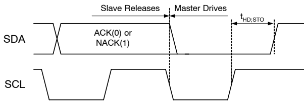
Figure 35. STOP Bit
